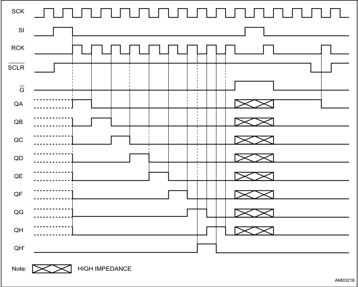
Figure 5. Timing chart
