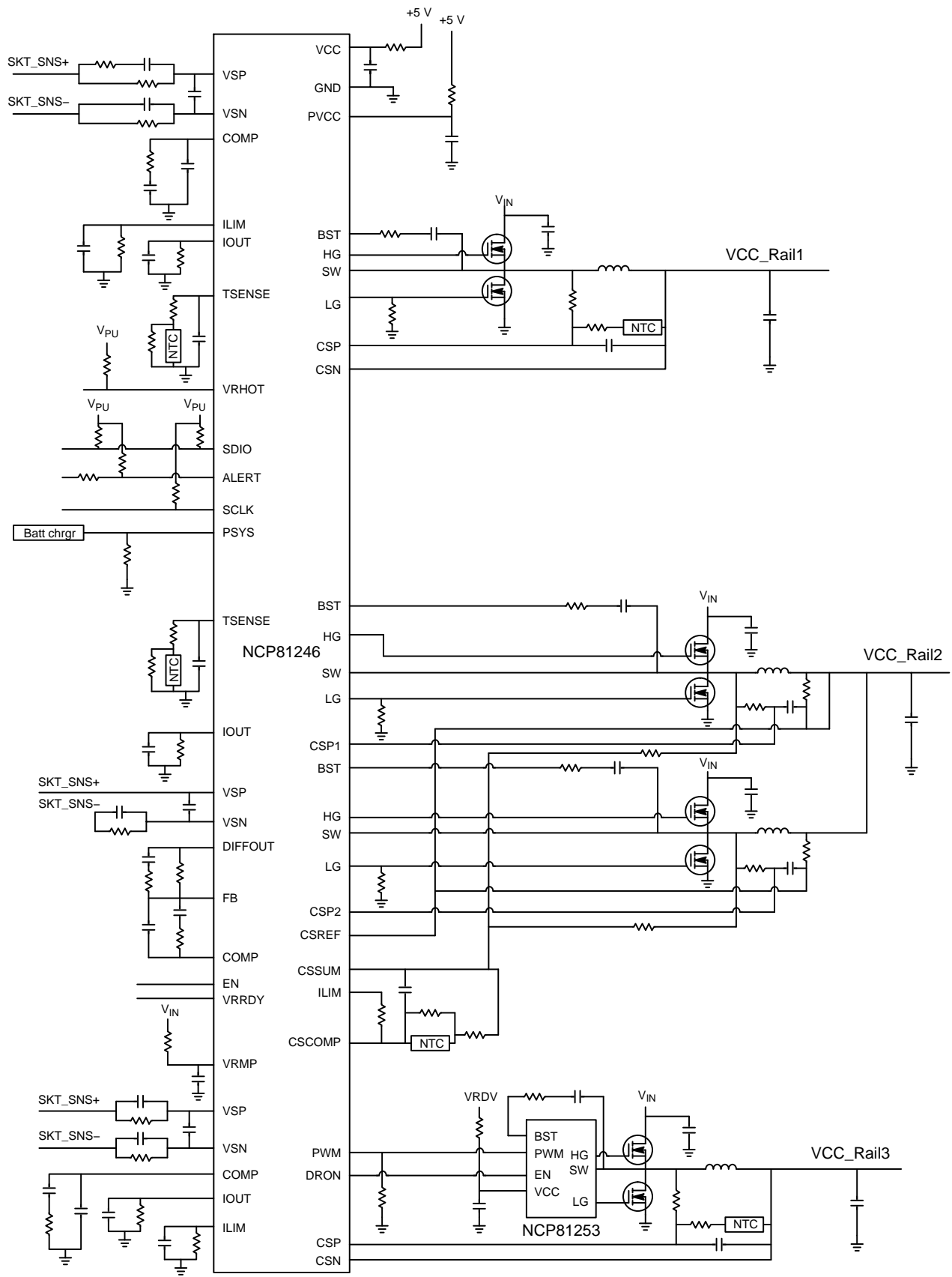
Figure 1. Application Schematic
