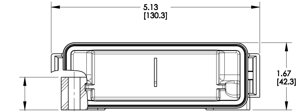
SECTION C-C
