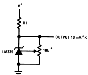
Figure 16. Calibrated Sensor
