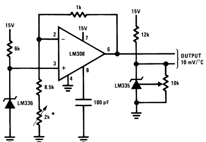
Figure 25. Centigrade Thermometer
