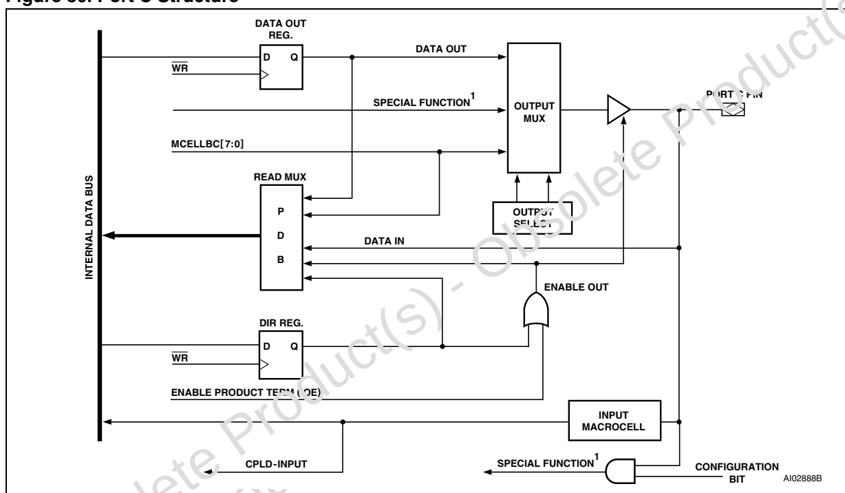
Figure 30. Port C Structure
