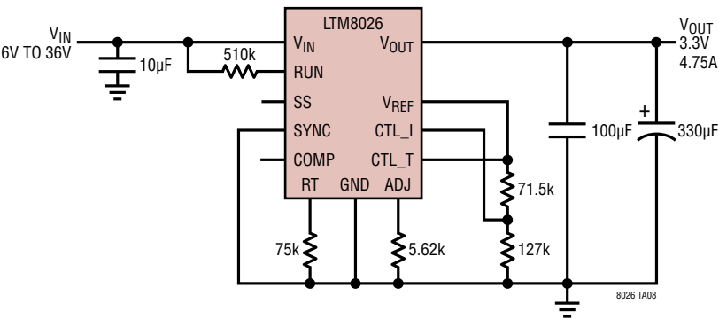
36V IN , 3.3V OUT Step-Down Converter with 4.75A Accurate Current Limit
