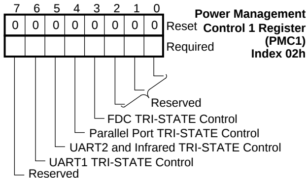
FIGURE 9-5. PMC1 Register Bitmap
