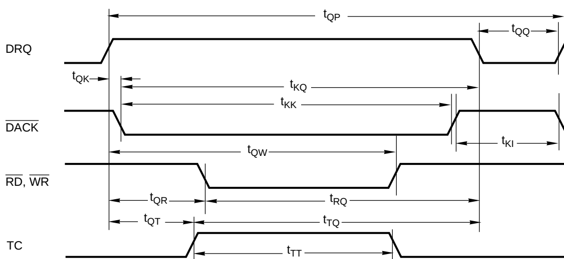
FIGURE 13-15. FDC DMA Timing
