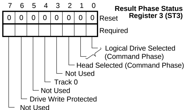
FIGURE 5-19. ST3 Result Phase Register
