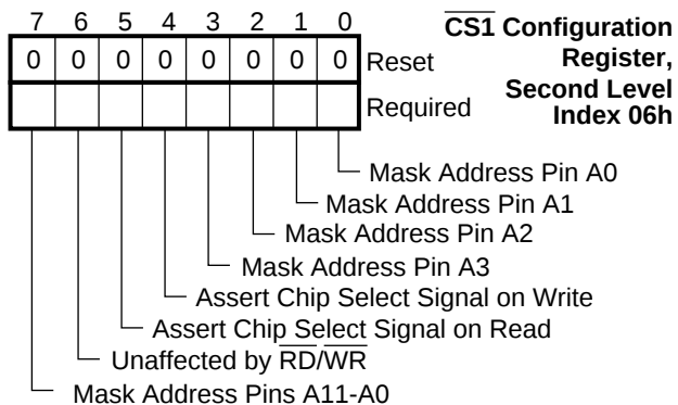
FIGURE 2-15. \overline{\text{CS1}} Configuration Register Bitmap
