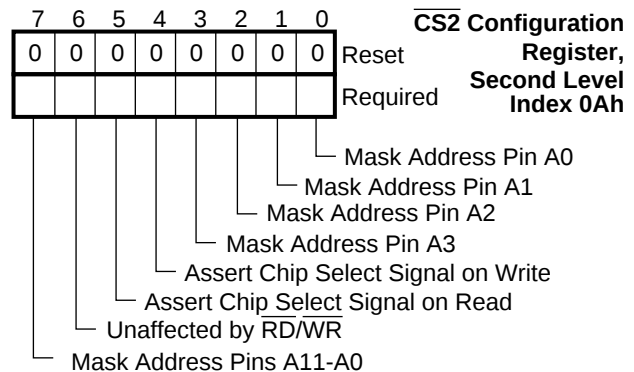
FIGURE 2-16. \overline{\text{CS2}} Configuration Register Bitmap
