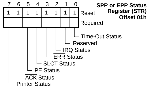
FIGURE 6-5. SPP or EPP STR Register Bitmap
