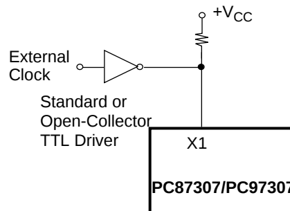
FIGURE 3-5. External Clock Connection
