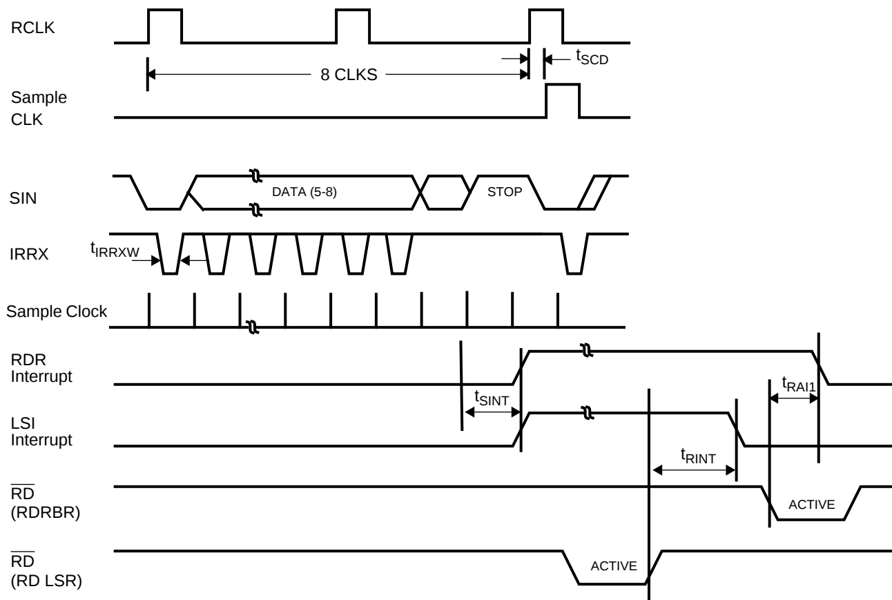
FIGURE 13-8. Receiver Timing
