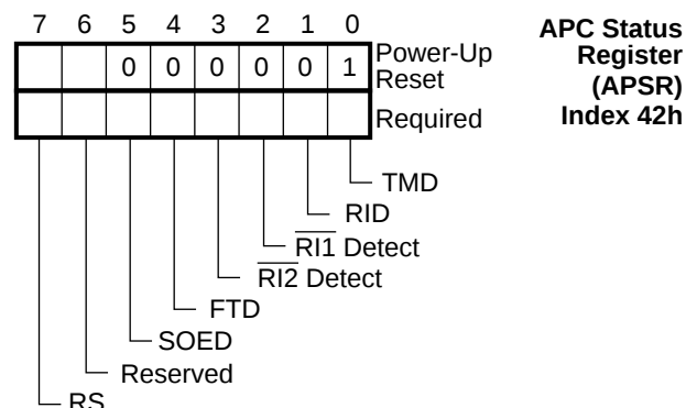
FIGURE 4-13. APSR Register Bitmap
