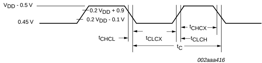
Fig 13. External clock timing.
