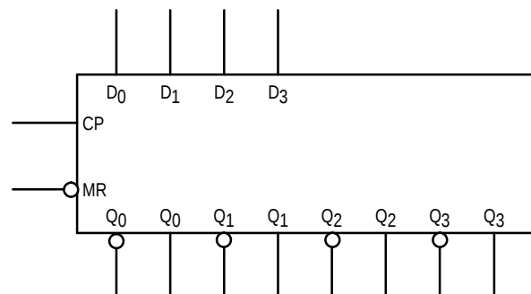
LOGIC SYMBOL
