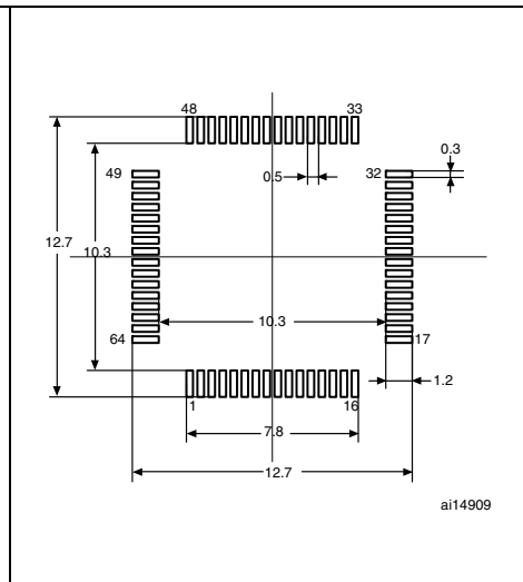
Figure 57. Recommended footprint (1)(2)
