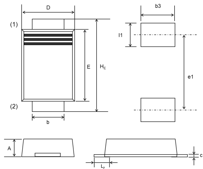
SOD-128, (PMD™)
