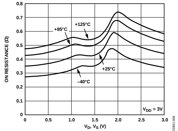
Figure 8. On Resistance vs. V_D , V_S for Different Temperatures, V_{DD} = 3\text{V}
