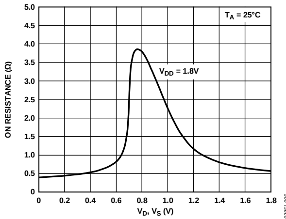
Figure 6. On Resistance vs. V_D , V_S ; V_{DD} = 1.8\text{V}
