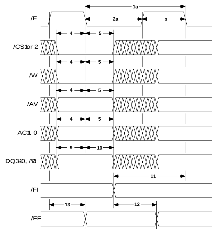
Figure 9: Write Cycle
