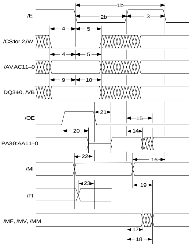
Figure 10: Compare Cycle
