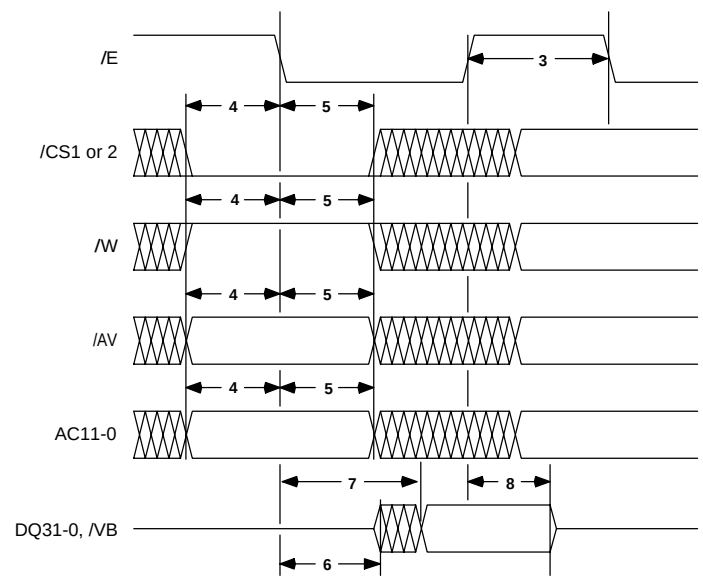
Figure 8: Read Cycle
