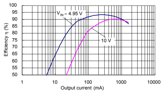
(8) S-8533A50AFT (Si3454DV/Si3455DV)
