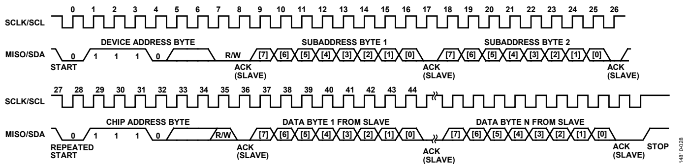
Figure 30. I 2 C Slave Burst Mode Read Operation (N Bytes)
