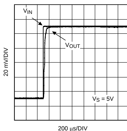
Figure 67. Step Response
