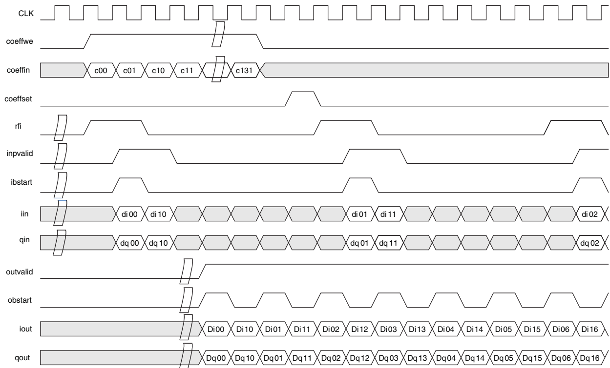
Figure 2-20. Multi-Channel (2 Channels) DHIGHSPEED I&Q Polyphase-Interpolator (1:4)
