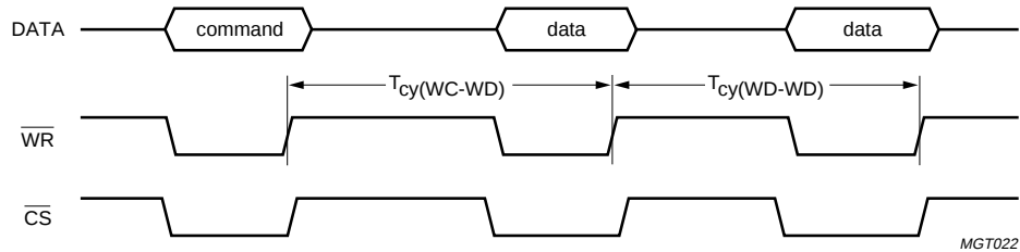
Fig 21. Write command + write data cycle timing.
