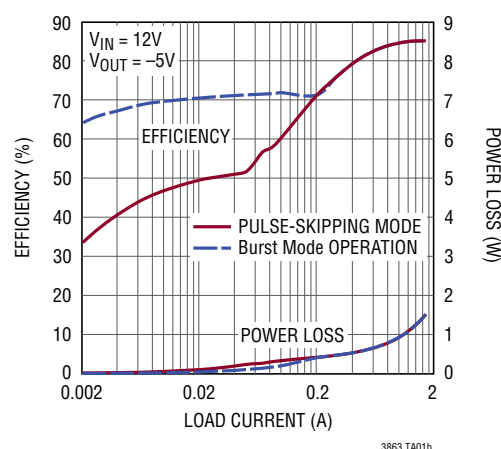
Efficiency
