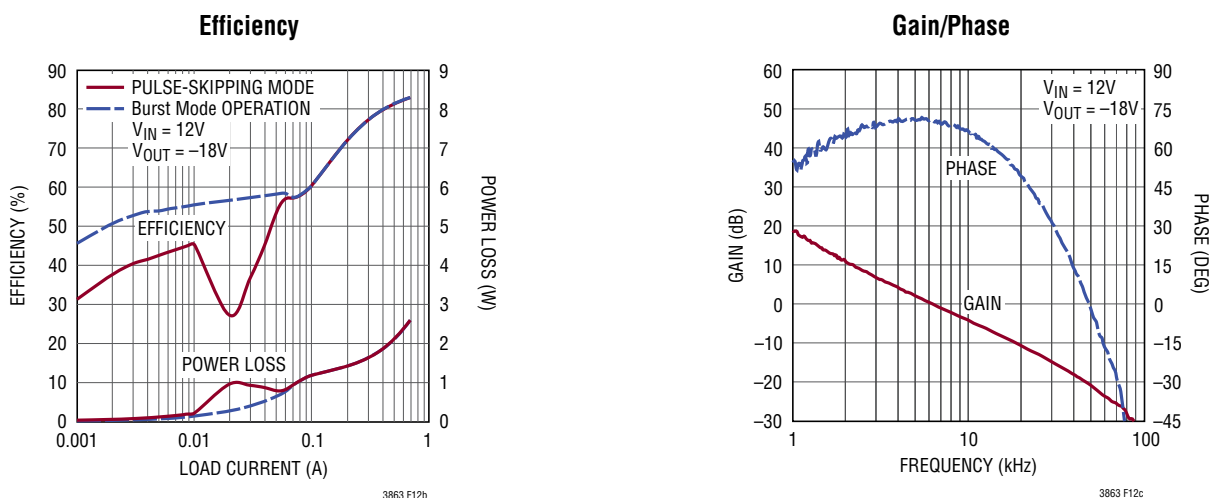
Figure 12. 5V to 23V Input, -18V/700mA Output, 750kHz Inverting Converter
