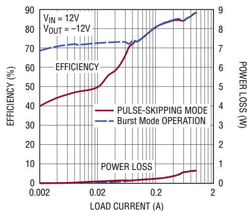
-12V Efficiency
