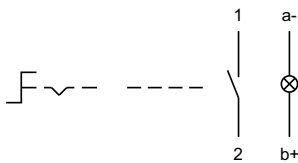
31 Selector switch 2 positions page 11 | Selector switch actuator 2 positions, flush mounting page 19
