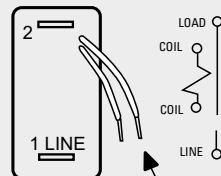
Relay Trip (Note A) Single Pole
