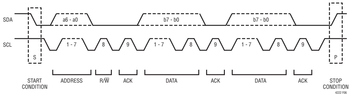
Figure 6. Data Transfer Over I 2 C or SMBus
