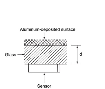
Fig 12. Light Current Measurement Setup Diagram
