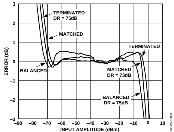
Figure 34. Comparison of Terminated, Matched, and Balanced Input Drive at 1.9 GHz
