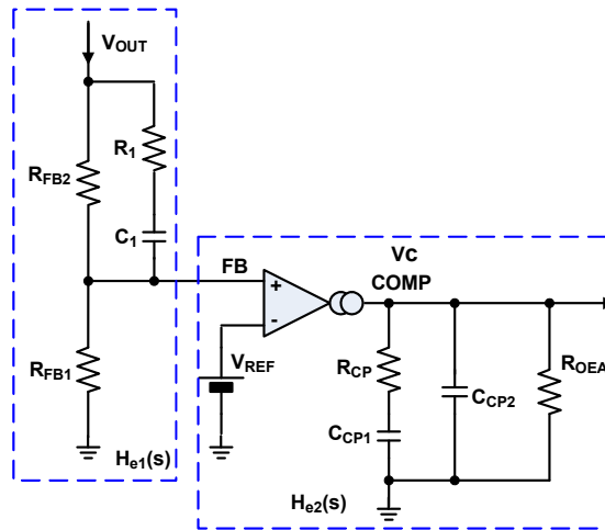
Figure 139. Type-3 Compensation
