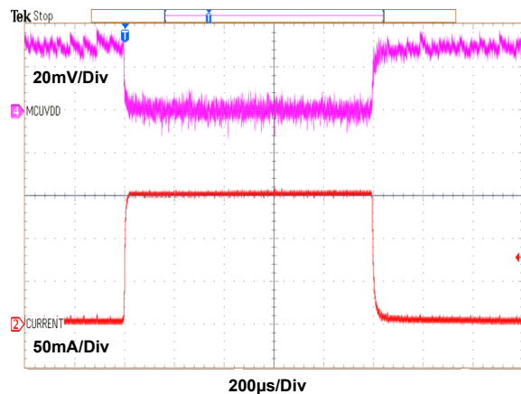
Figure 71. MCULD0 Load Transient, I_{LOAD} = 0 to 150mA, MCULD0 Offset = 5.0V
