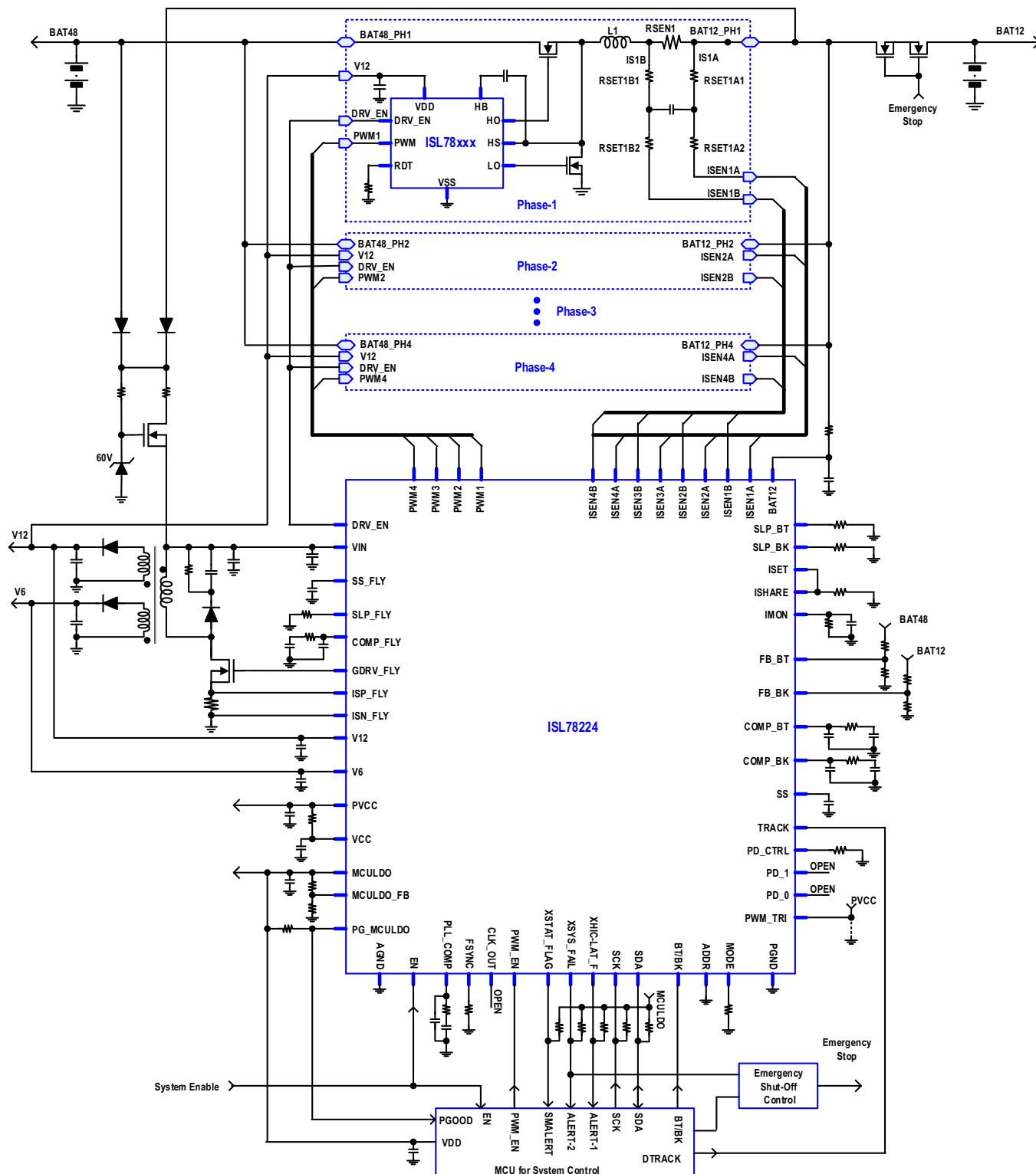
Figure 4. 4-Phase Synchronous Bidirectional Converter with Single Device Configuration
