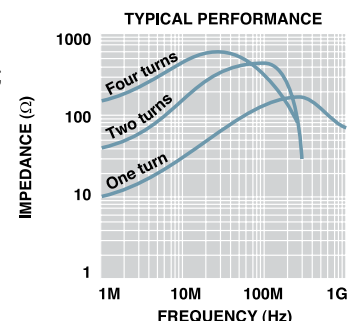
fig. 4 Increased impedance; multiple turns ( N^2 ) vs. one turn through ferrite; i.e., 2 turns ( 2^2 ) = 4 times impedance
