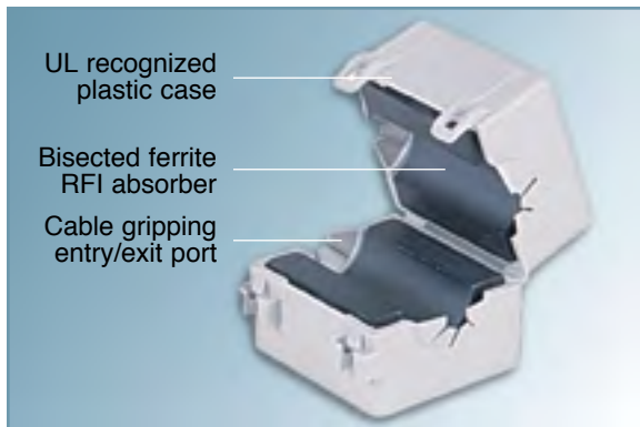
Typical FerriShield RFI suppressor.
