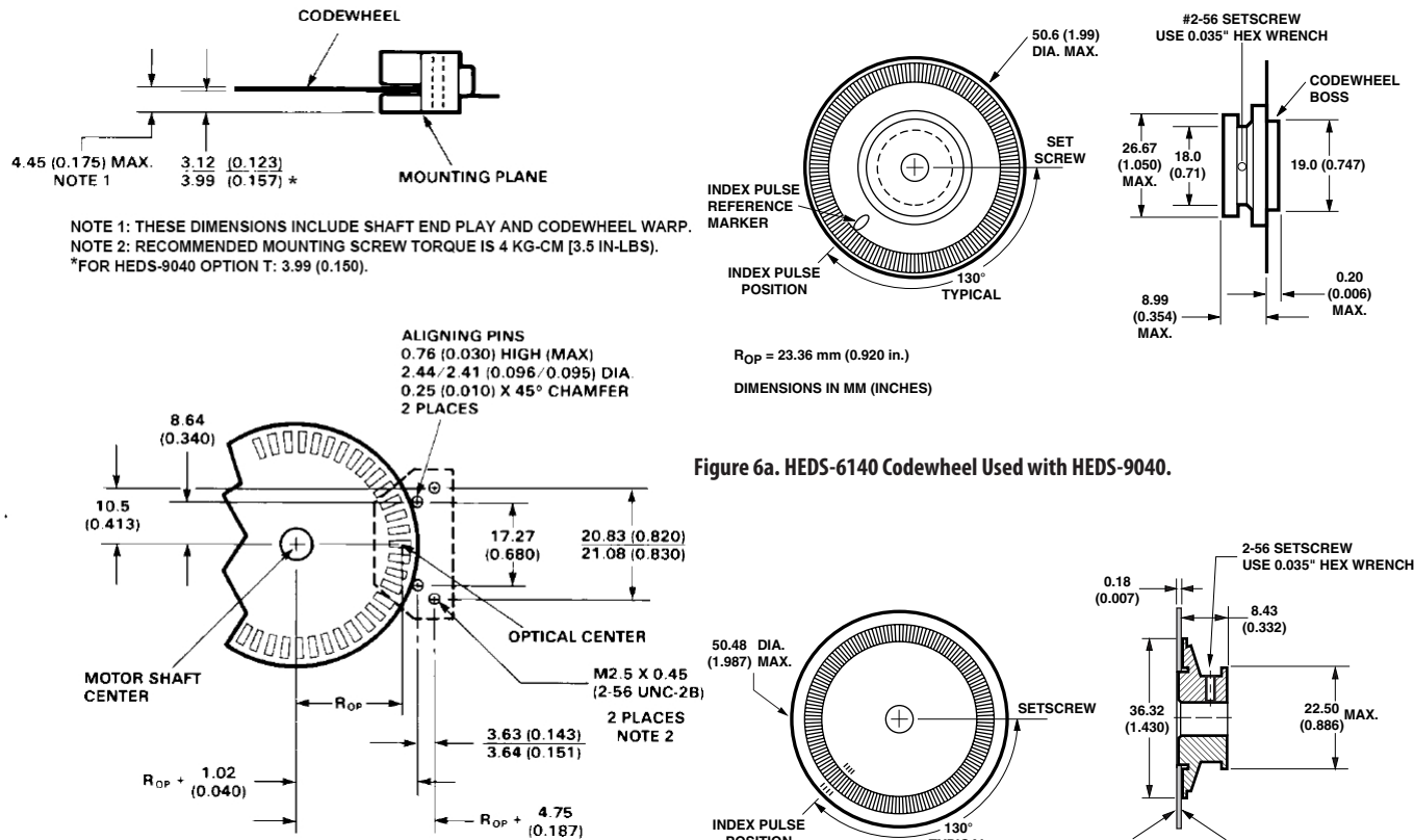
Figure 5. Mounting Plane Side A.
