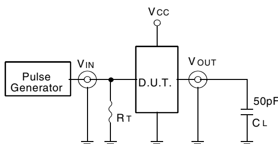
Fig. 4: C_L = 50\text{pF} Circuit
