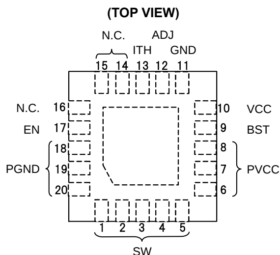
Figure 2. Pin Configuration
