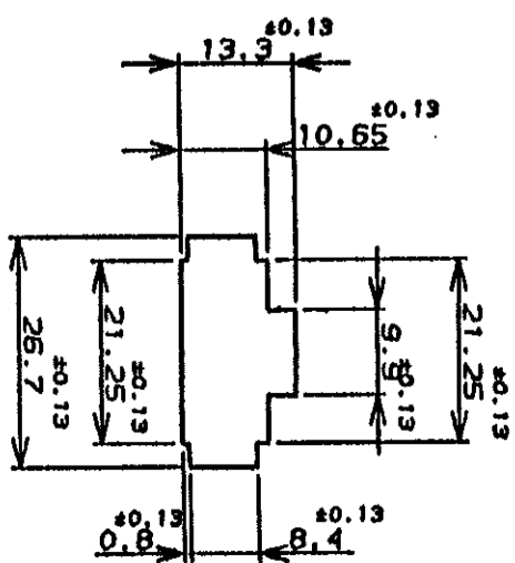
コネクタ取付穴寸法 (FIG. 1) RECOMMENDED PANEL OPENING DIMENSION
