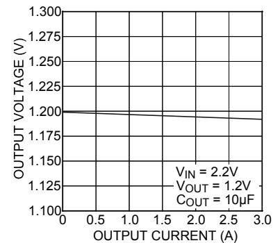
Load Regulation
