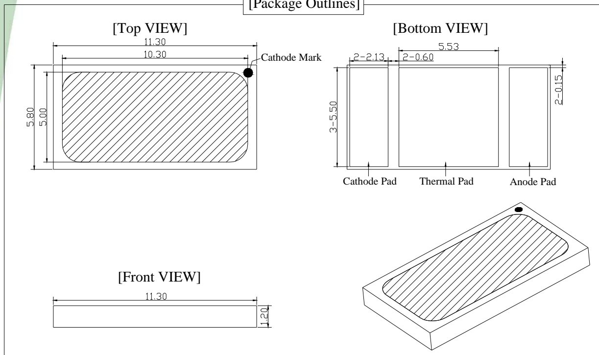
[Package Outlines]
