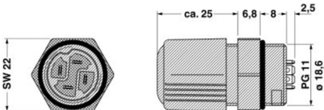
Dimensioned drawing
