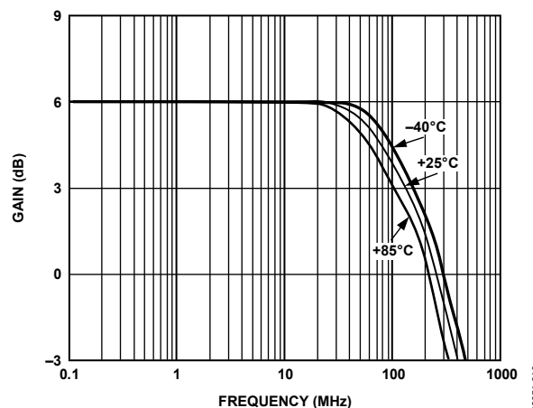
Figure 16. Frequency Response vs. Temperature, Gain = +2, V_S = \pm 5\text{ V} , V_{OUT} = 2\text{ V p-p}
