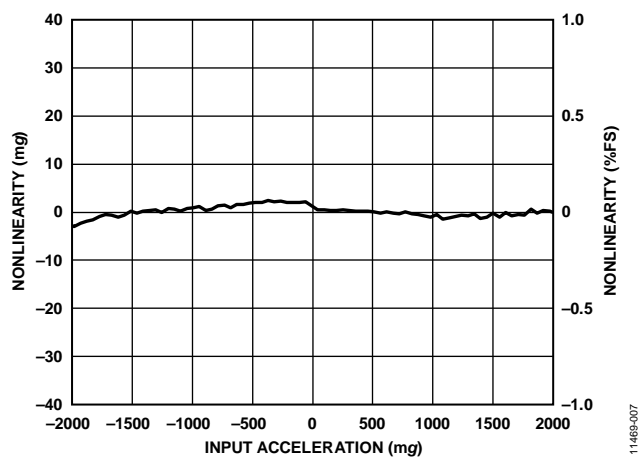
Figure 7. Y-Axis Nonlinearity, \pm 2 g Input Range
