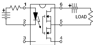
"B" Connection
