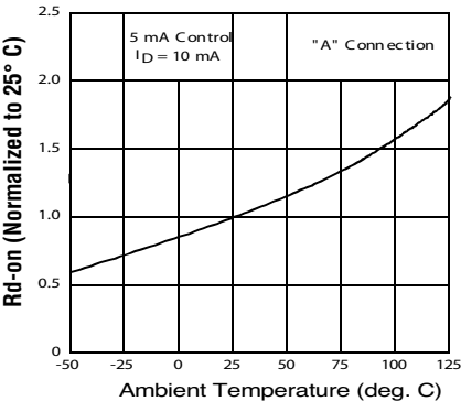
Figure 4. Typical Normalized On-Resistance
