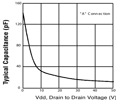
Figure 9. Typical Output Capacitance
