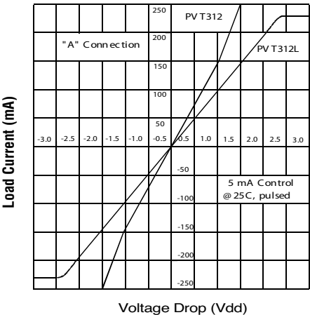
Figure 3. Linearity Characteristics
