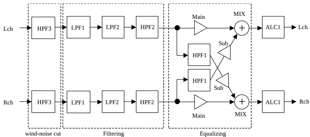
Figure 21. Digital EQ/HPF/LPF
