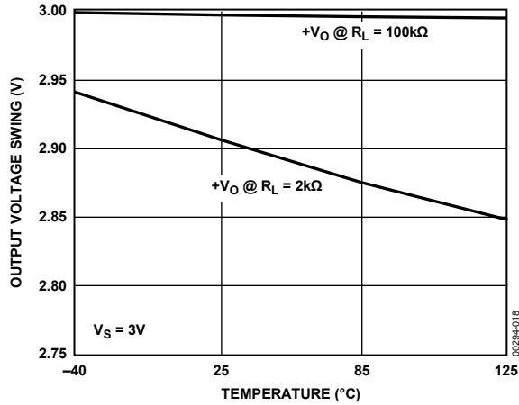
Figure 13. Output Voltage Swing vs. Temperature, V S = 3 V
