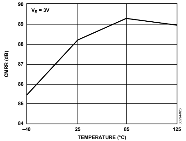
Figure 18. CMRR vs. Temperature, V_S = 3V
