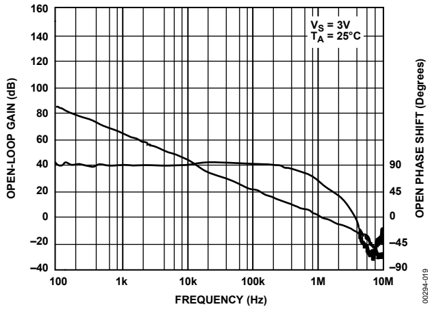
Figure 14. Open-Loop Gain and Phase vs. Frequency, V_S = 3V
