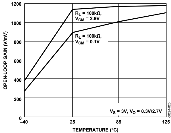
Figure 15. Open-Loop Gain vs. Temperature, V_S = 3V
