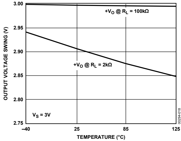
Figure 13. Output Voltage Swing vs. Temperature, V_S = 3V
