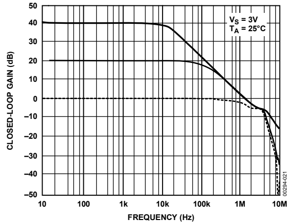
Figure 16. Closed-Loop Gain vs. Frequency, V_S = 3V
