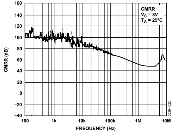
Figure 17. CMRR vs. Frequency, V_S = 3V
