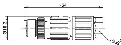
Dimensional drawing
