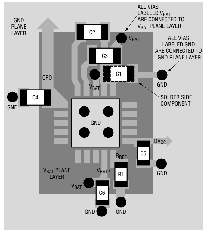
Figure 7. PC Board Layout Example (LTC3209-1)
