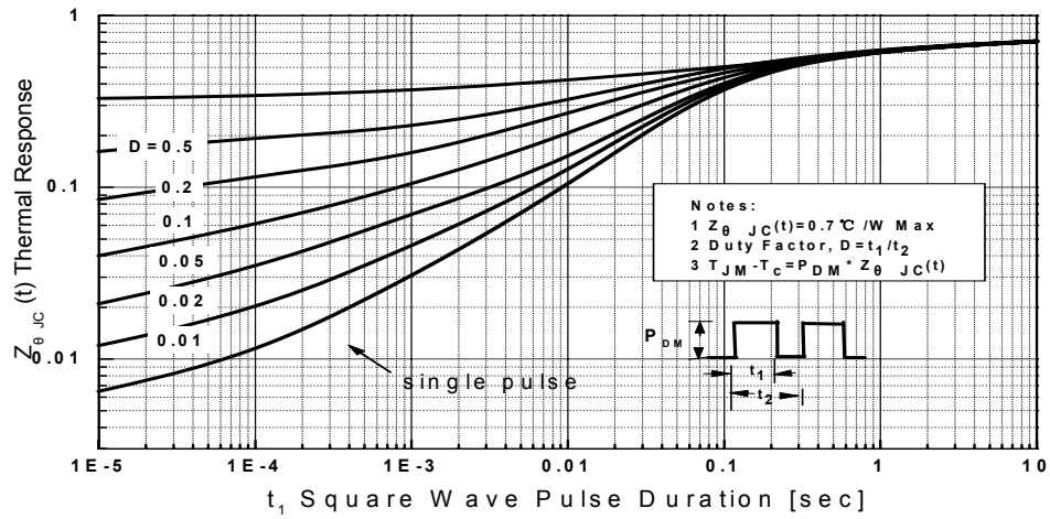
Transient Thermal Response Curve For JCS10N65CT
