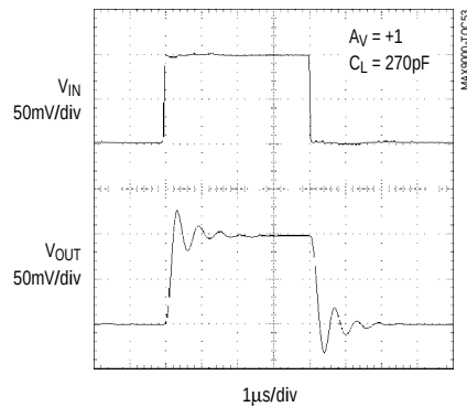
MAX9000/MAX9001/MAX9002 OP-AMP SMALL-SIGNAL TRANSIENT RESPONSE WITH CL
