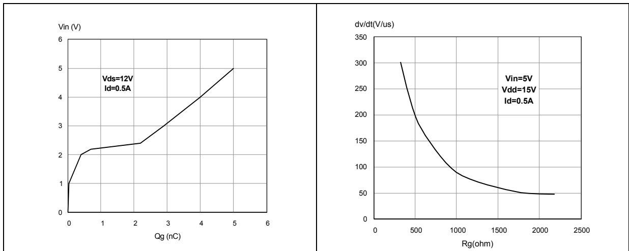
Figure 20. Turn-off drain source voltage slope (part 1/2)
