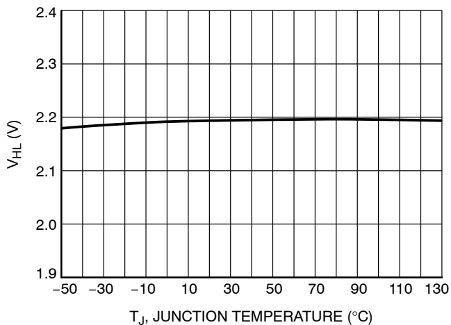
Figure 55. Comparator Threshold for Line Range Detection, V_{SENSE} Rising vs. Temperature
