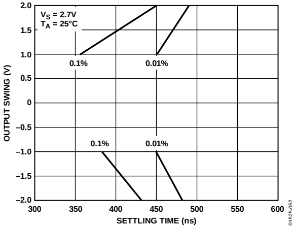
Figure 52. Output Swing vs. Settling Time
