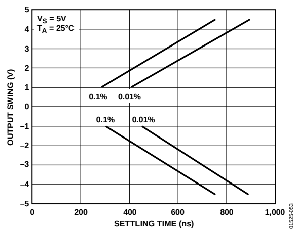
Figure 53. Output Swing vs. Settling Time
