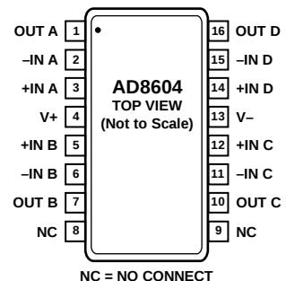
Figure 4. 16-Lead Shrink Small Outline QSO (RQ Suffix)
